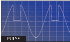
Voltage Harmonic & Interharmonics Test
