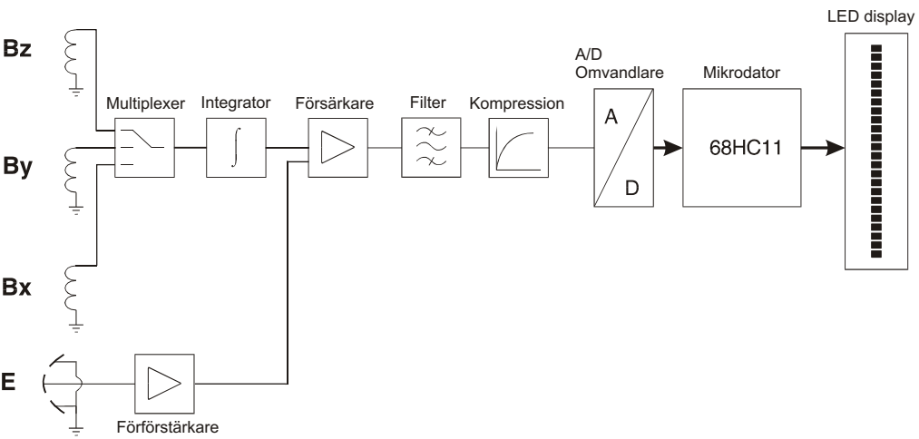
Fig. 4.2 FD2 blockdiagram
